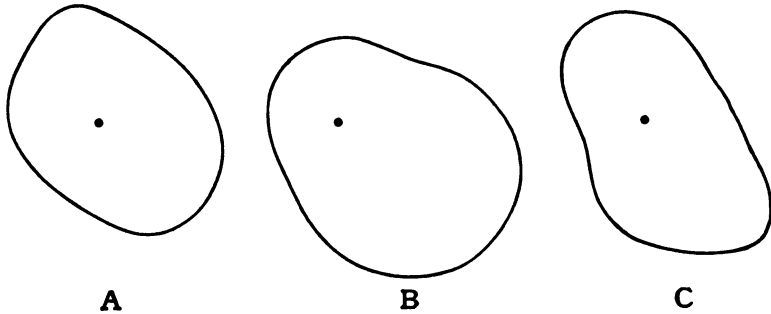
FIG. 14.—Mean Proper Motion Curves.
